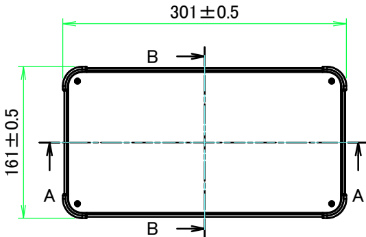
E view
